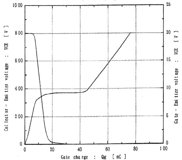
[ Inverter ] Dynamic Gate charge (typ) V_{CC} = 800\text{V} , I_c = 10\text{A} , T_j = 25^\circ\text{C}
