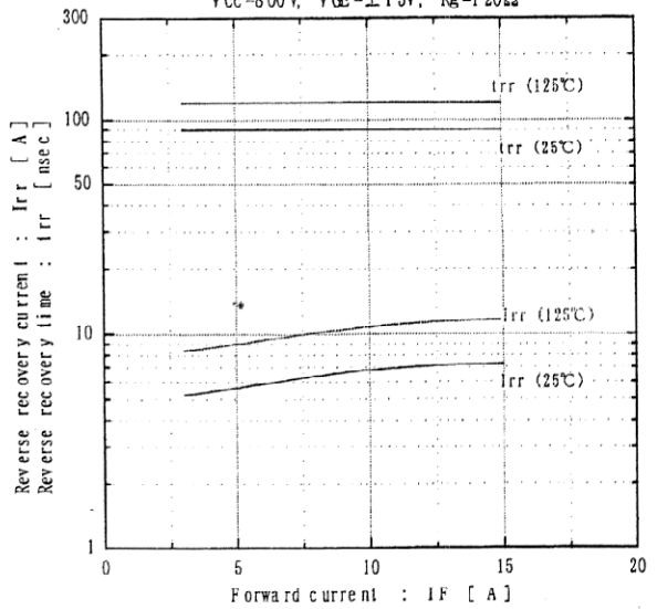
[ Inverter ] Reverse recovery characteristics (typ.) V_{CC}=8.00V, V_{GE}=\pm 15V, R_g=120\Omega
